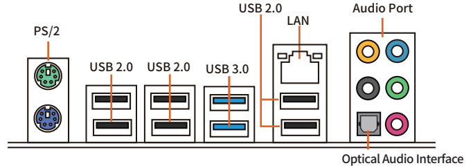
1-2 Overall Rear I/O Panel Display
