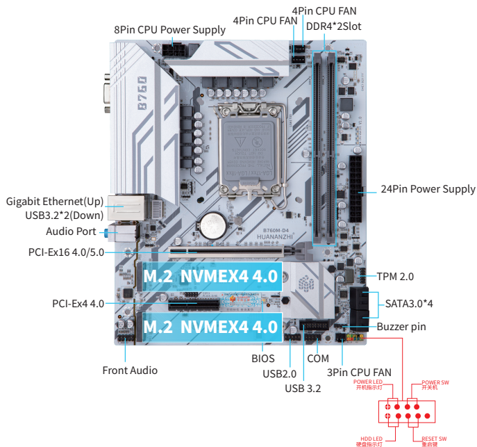
1-1 B760M-D4 Motherboard Illustration
