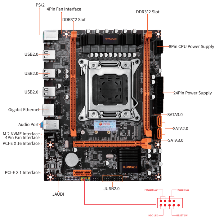
1-1 X79-4M V2.0 Motherboard illustration
