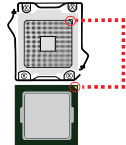
2-6 CPU Installation
