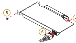
2-10 Graphics Card Installation
