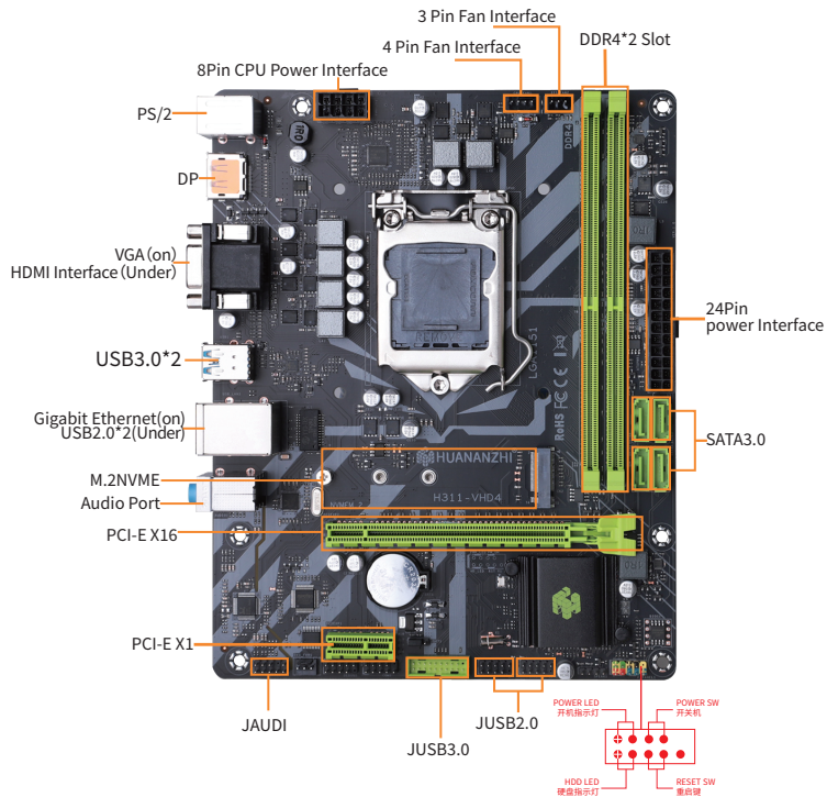
1-1 H311-VHD4 MotherBoard Illustration
