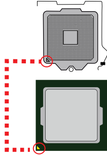
Figure 2-7 CPU installation
