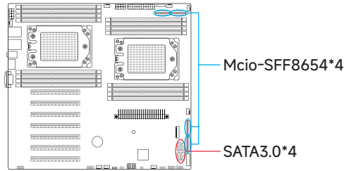
2 -10 SATA Interface
