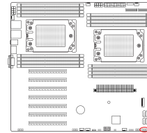
2-3 PCI Expansion Slot
