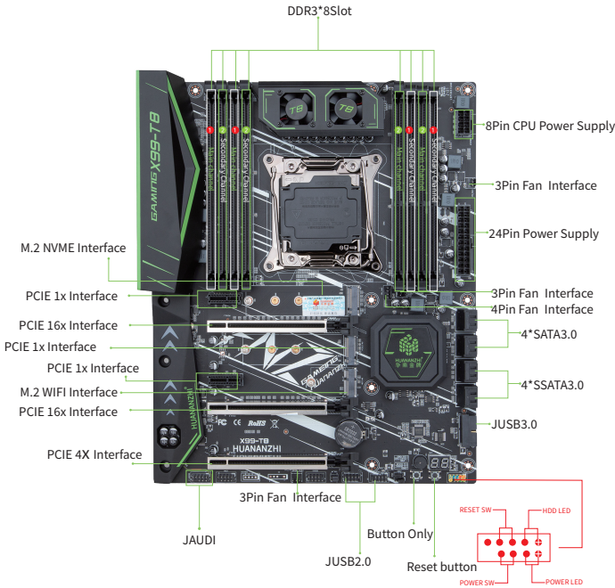
1-1 X99-T8 Gmotherboard Illustration
