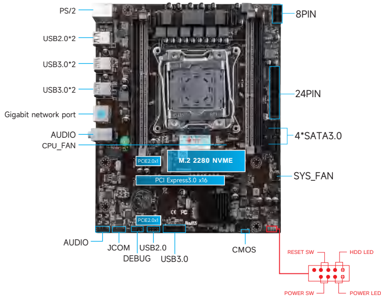
1-1 X99-MTF Motherboard Illustration
