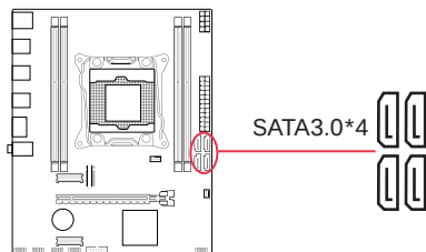
2 -10 SATA Interface
